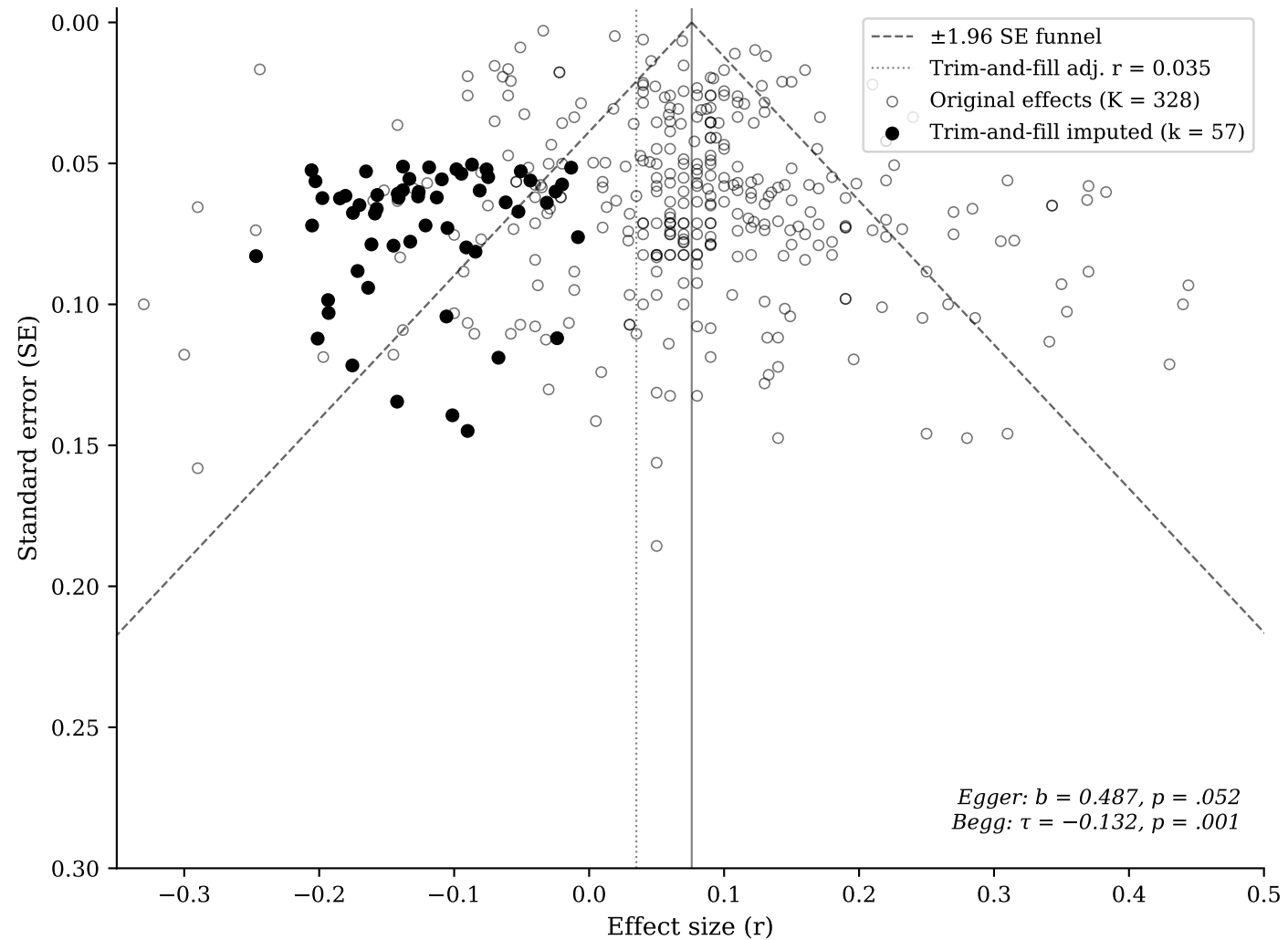
Figure 5. Funnel Plot with Trim-and-Fill Correction k = 57 imputed; adj. r = 0.035 [0.018, 0.051]
