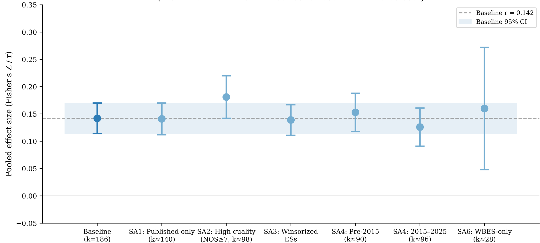
Figure 4. Sensitivity Analysis — Robustness of Pooled I→P Effect (Framework validation — illustrative based on simulated data)
