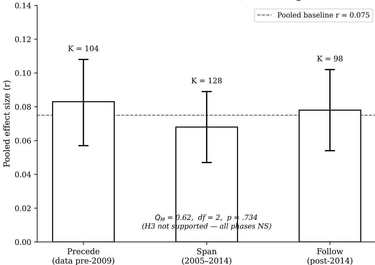
Figure 3. DPL Phase Moderation of I→P Effect (Actual results: PRE > FOL > SPN, all non-significant)
