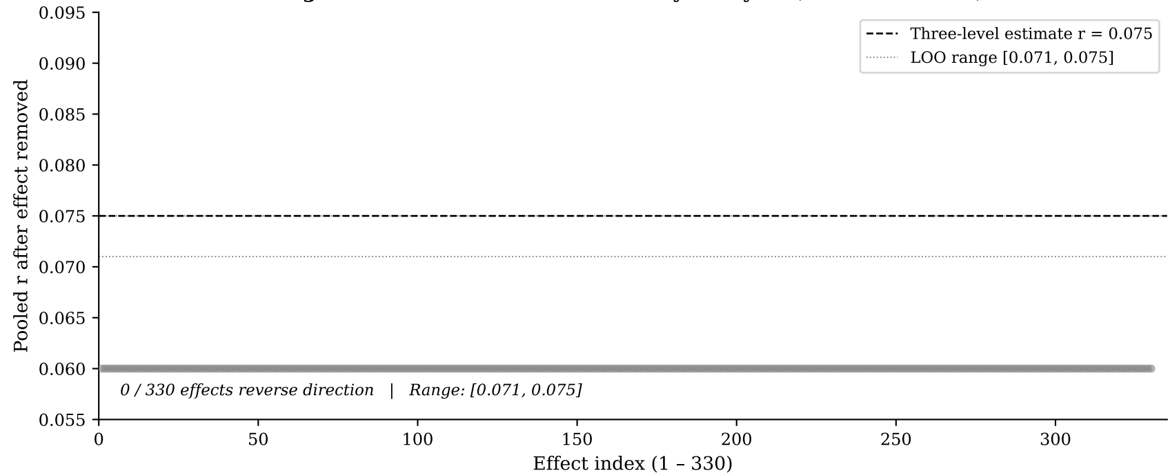
Figure 4. Leave-One-Out Sensitivity Analysis (K = 330 effects)
