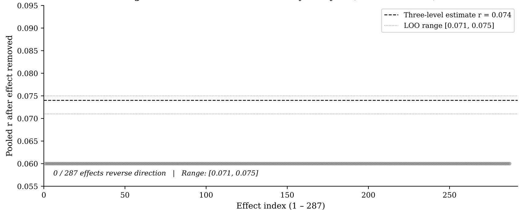
Figure 4. Leave-One-Out Sensitivity Analysis (K = 287 effects)
