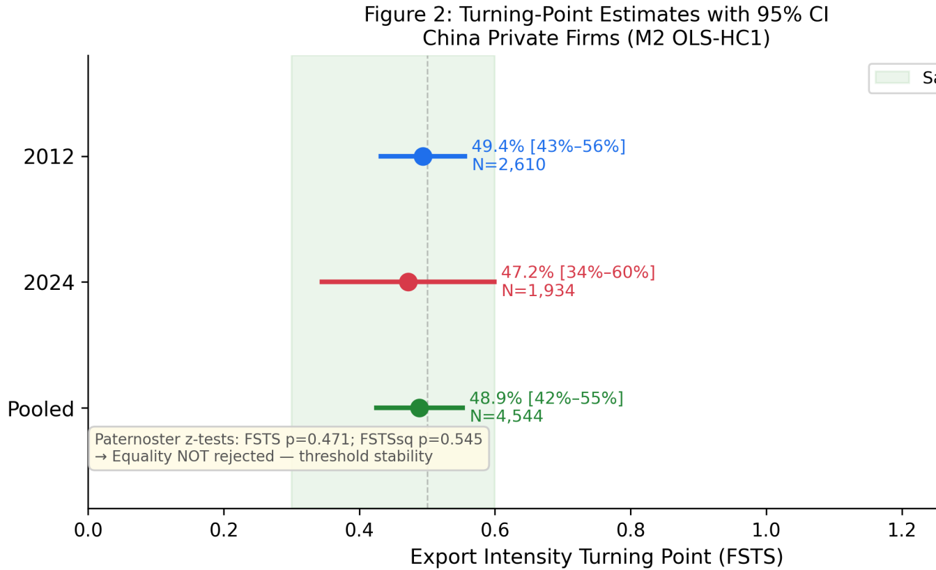
Figure 2. Delta-method 95 % confidence intervals for the turning-point estimates in 2012 (49.4 %) and 2024 (47.2 %). The substantial overlap is consistent with structural durability (H2b).
