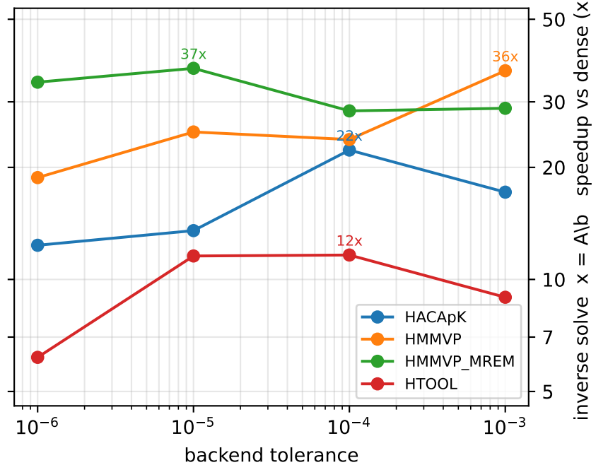
inverse solve x = A \backslash b (GMRES) (dense: 3.0 h, 4969 its)
