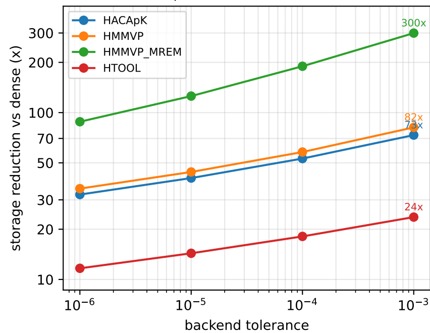
compression (dense: 525.1 GB)
