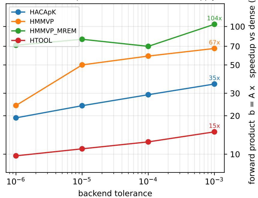
matvec: forward product b = A \times (dense: 2.13 s/apply)
