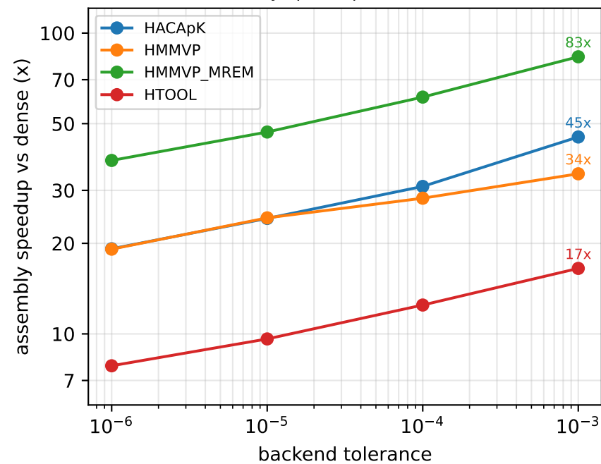
assembly speedup (dense: 1.9 h)
