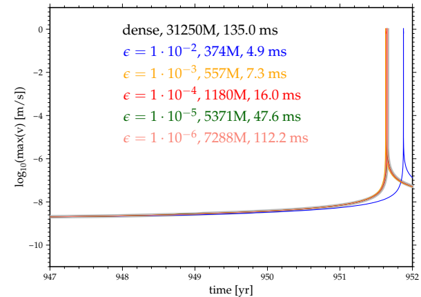
HMMVP, 0.25km, N = 64000
