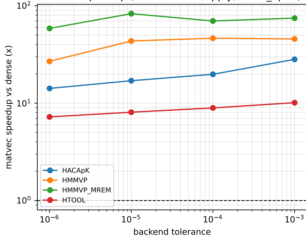
matvec speedup (dense: 2.17 s/apply, meas_np64)
