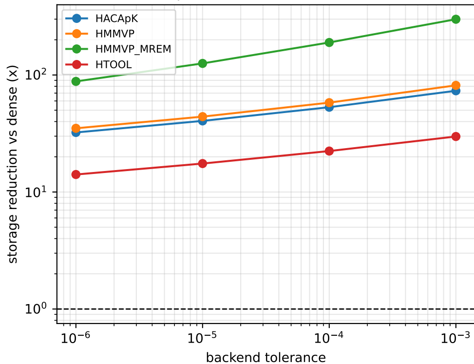
compression (dense: 525.1 GB)
