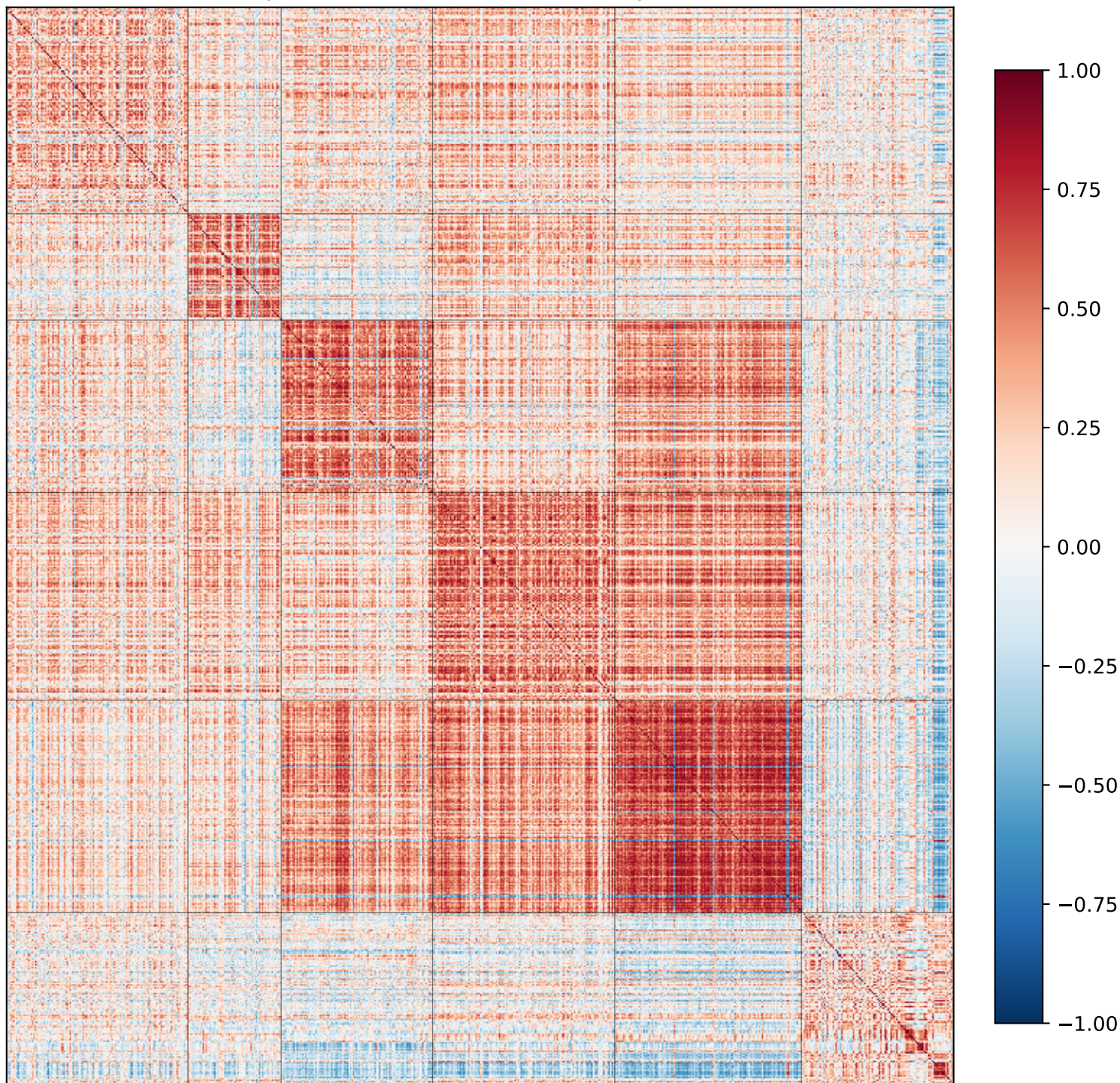
Family correlation matrix (ordered by module)
