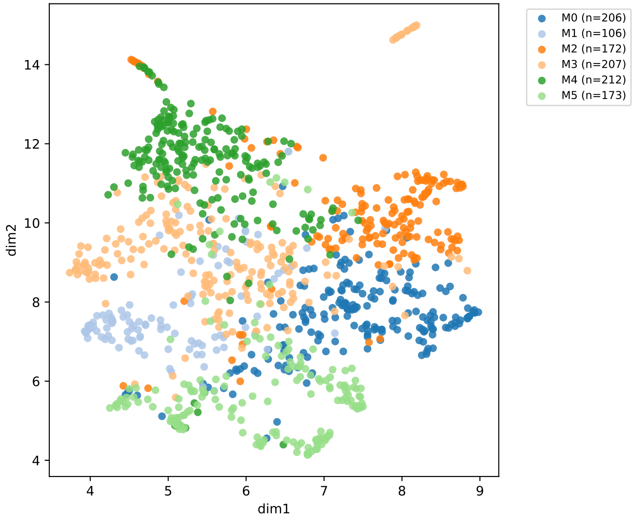
UMAP scatter (dim1 vs dim2) colored by module
