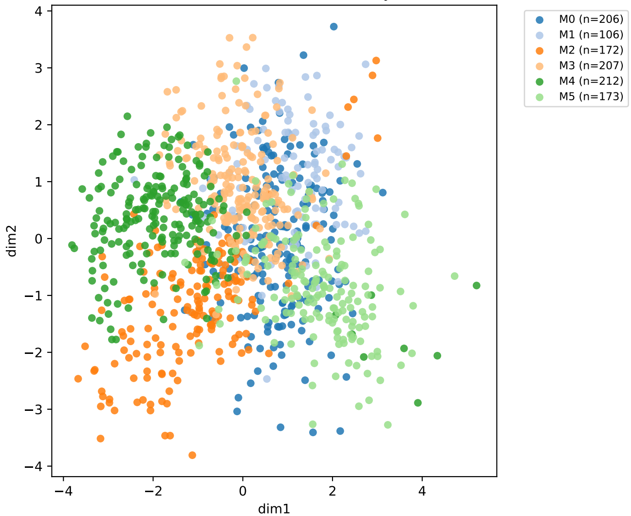
PCA scatter (dim1 vs dim2) colored by module
