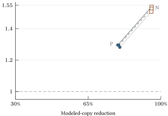
(a) Cholesky
