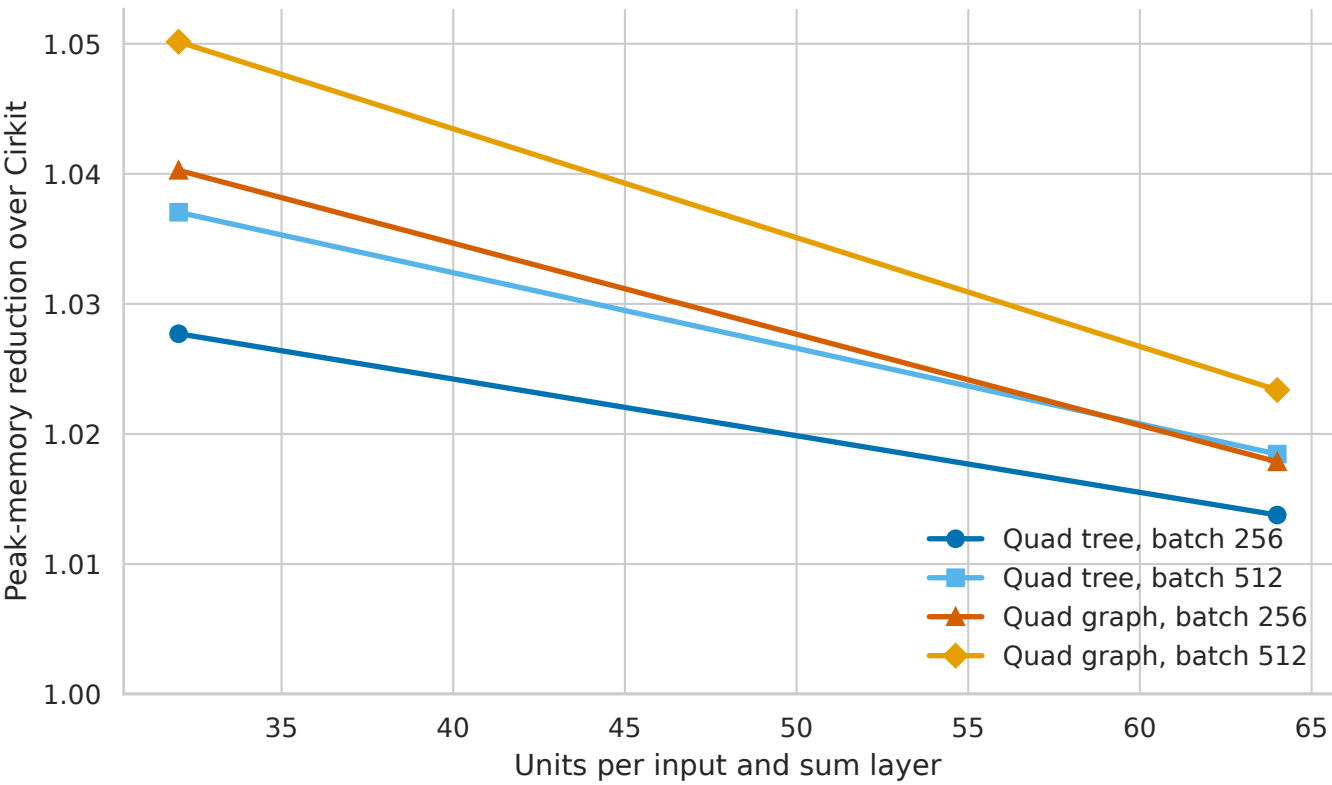
Extended Einsum Peak-Memory Reduction
