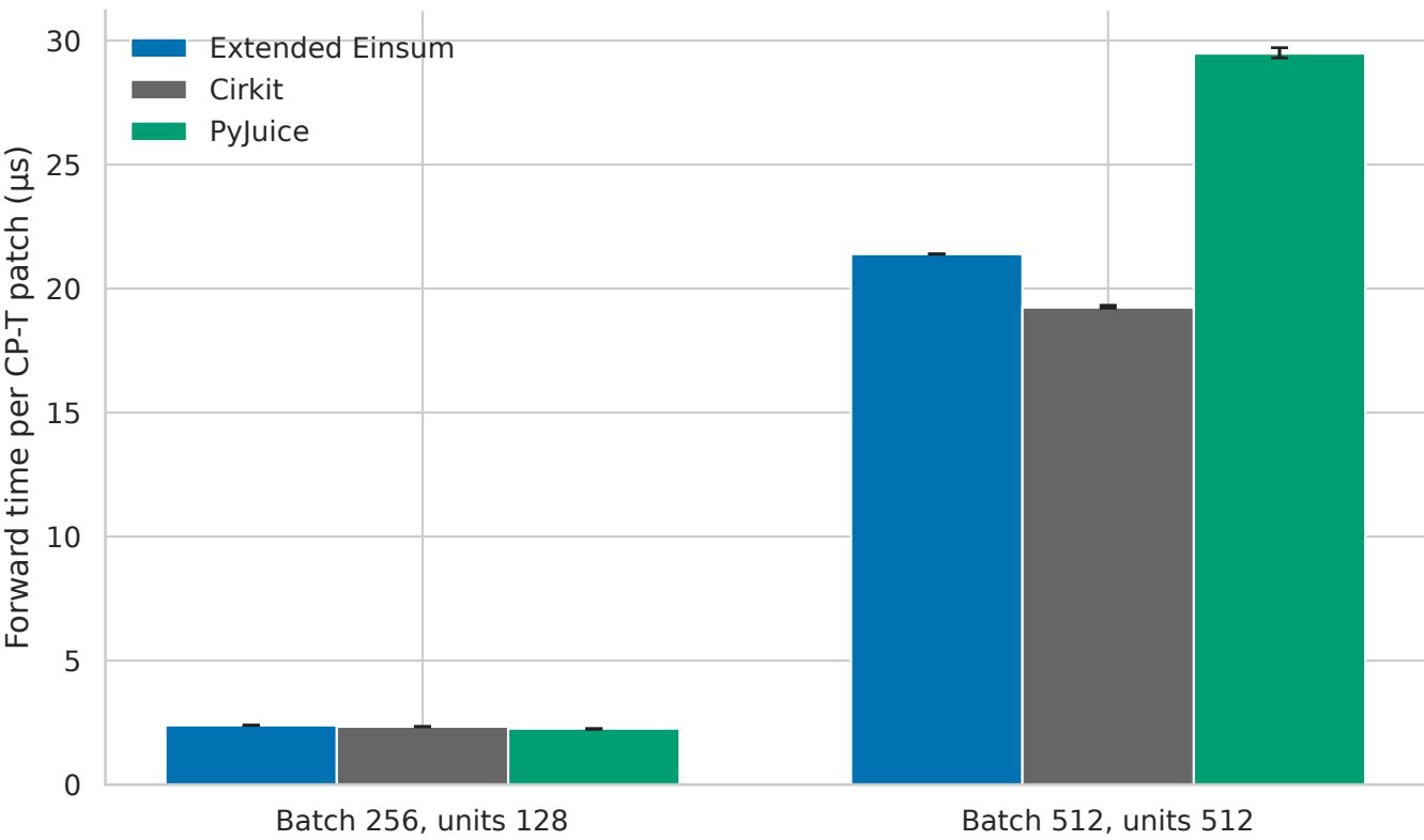
Parameter-Matched CP-T Forward Pass
