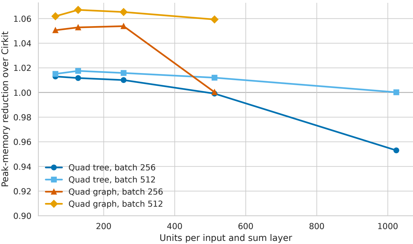
Extended Einsum CP Peak-Memory Reduction
