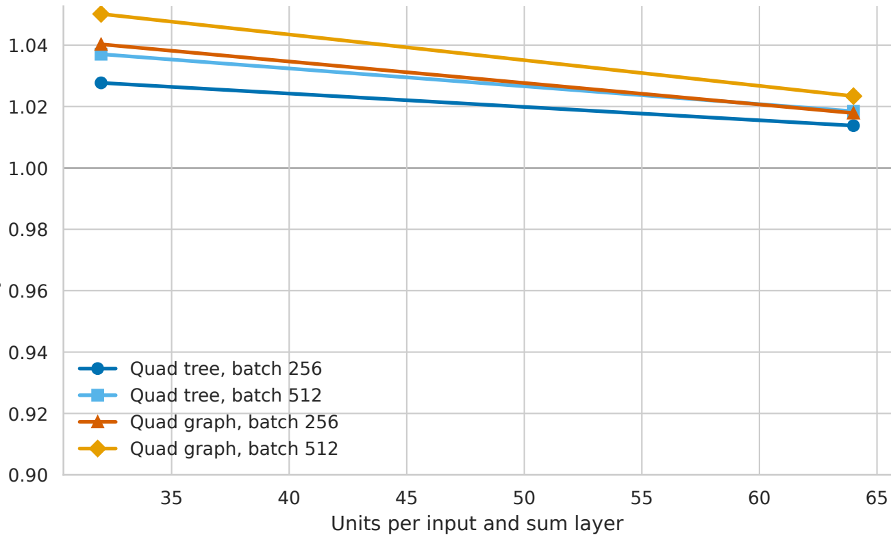
Extended Einsum Tucker Peak-Memory Reduction
