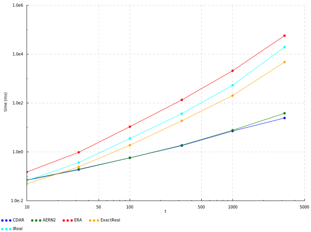
Figure 23: Benchmarks for loop of wait statements, evaluated at n = 1000 , scaled logarithmically
