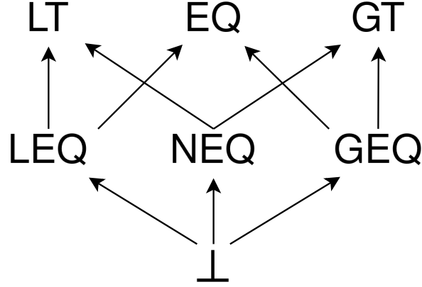
Figure 4: Hasse diagram of the ordering domain. Each arrow a \rightarrow b represents the relationship a \sqsubseteq b . Relationships inferrable through reflexivity or transitivity are omitted.
