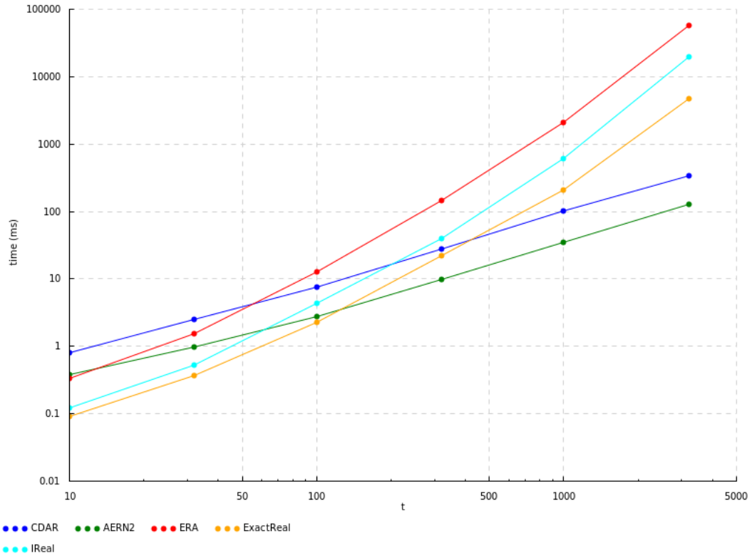
Figure 22: Benchmarks for a hybrid program that calculates sum of \lfloor t \rfloor + 1 elements, evaluated at n = 1000 , scaled logarithmically
