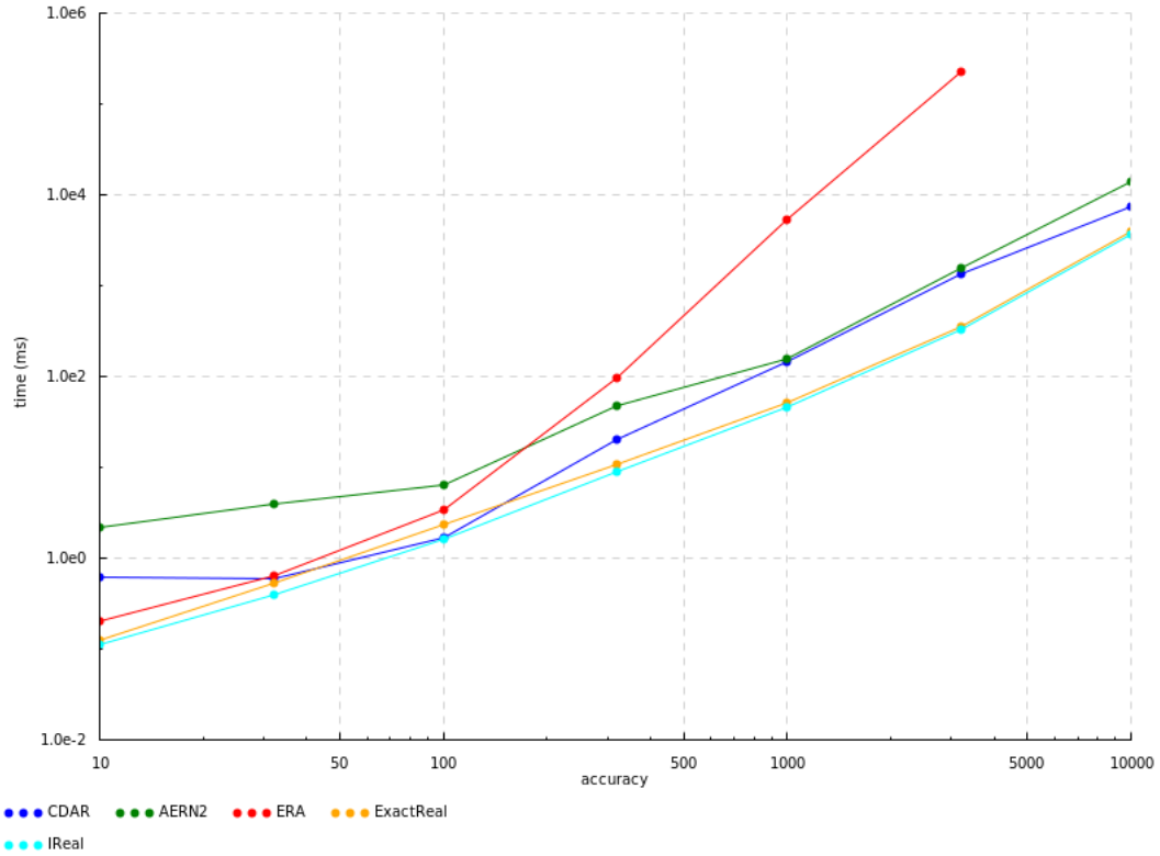
Figure 24: Benchmarks for ODE solver ( x'(t) = x(t) ) at t = 0.4 , scaled logarithmically
