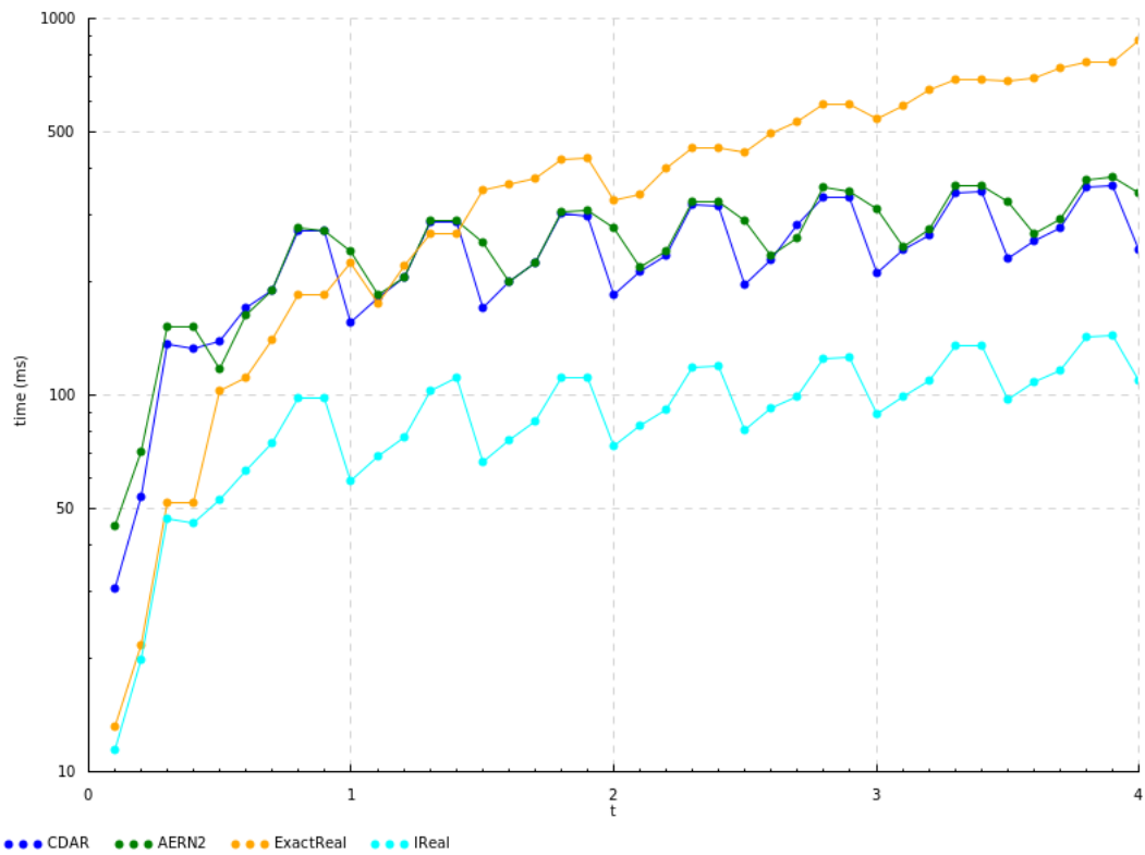
Figure 25: Benchmarks for ODE solver ( x'(t) = x(t) ) for n = 1000 , scaled logarithmically in the y-axis
