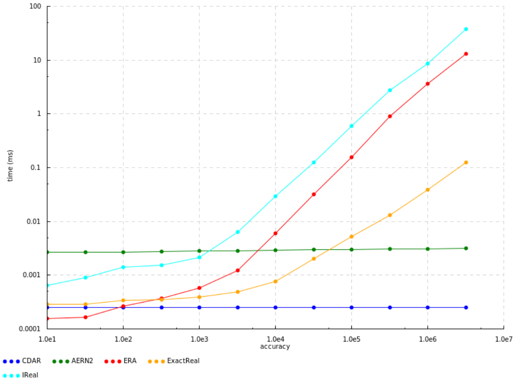
Figure 11: Benchmarks for fromInteger 1 , scaled logarithmically
