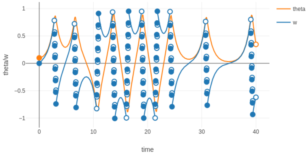
Figure 29: Plot of inverted pendulum program run in Lince
