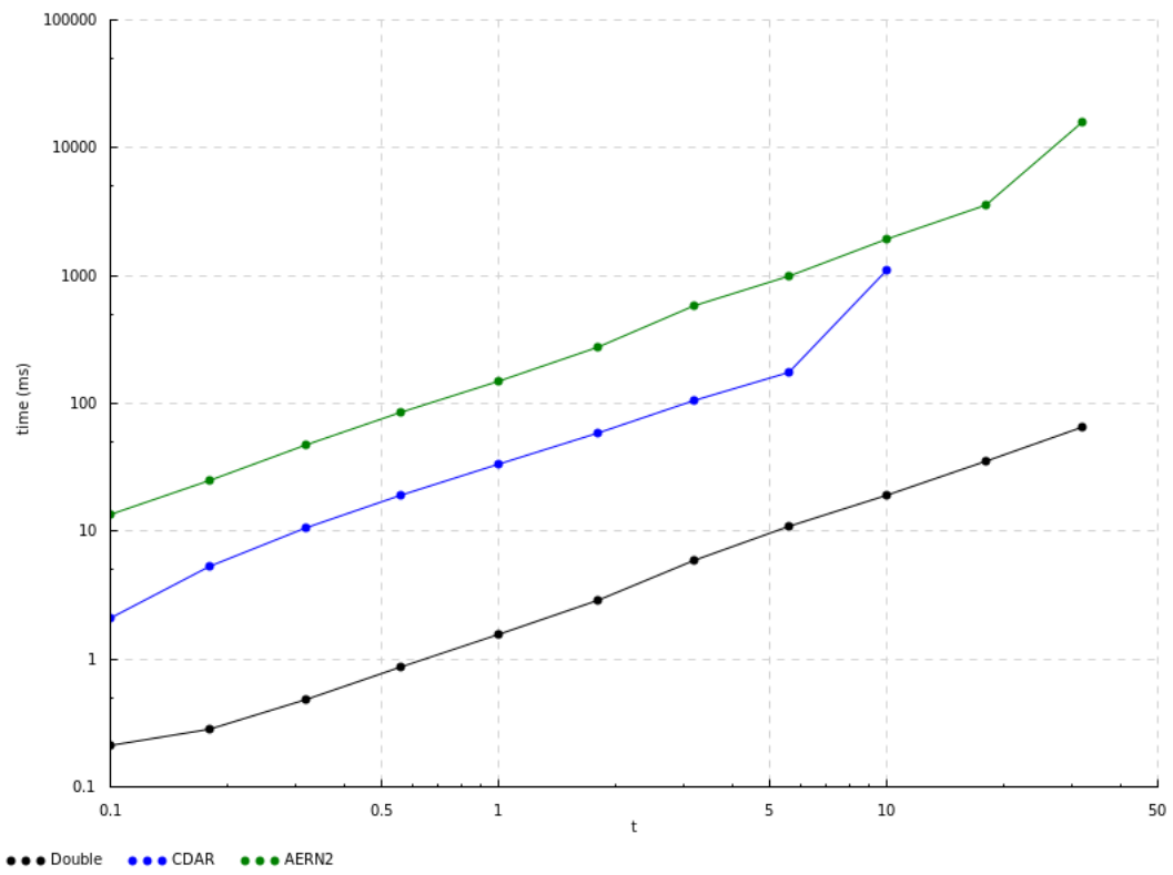
Figure 30: Benchmarks for inverted pendulum program ( n = 32 ), scaled logarithmically
