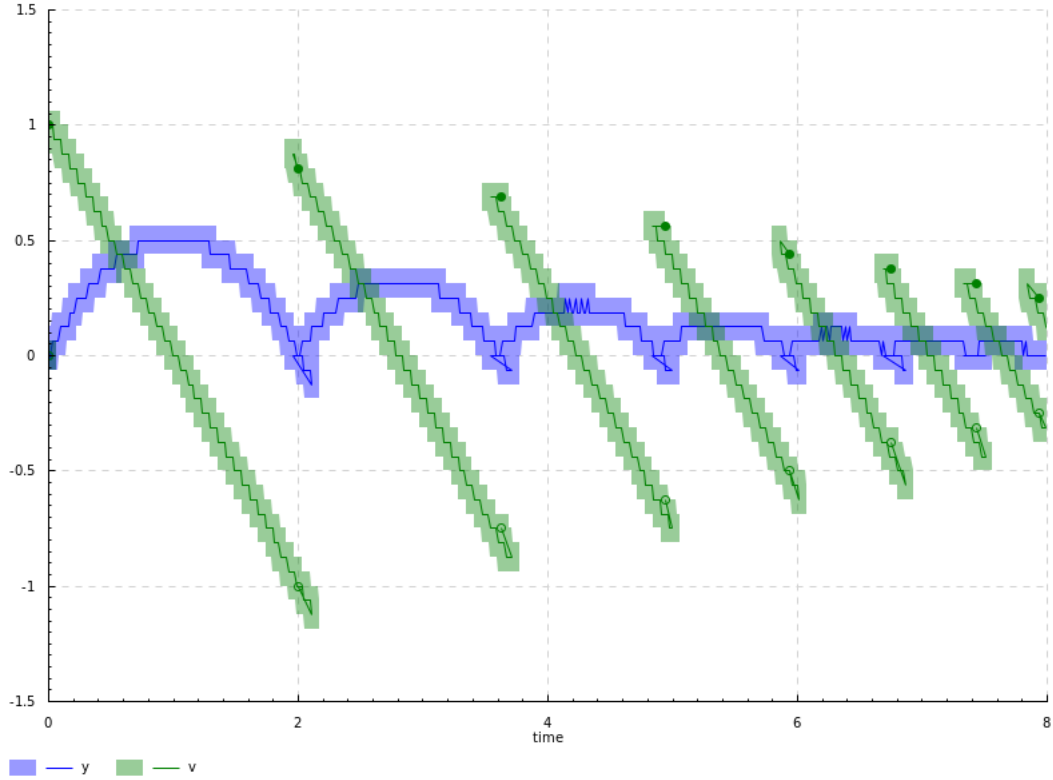
Figure 8: Plot of a Jaguar program with an accuracy of n = 4
