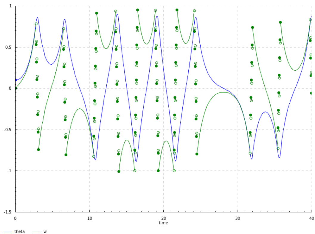
Figure 28: Plot of inverted pendulum program run with doubles
