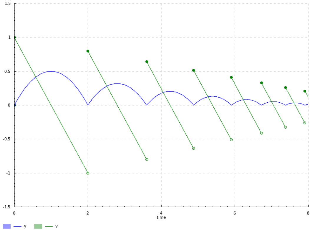
Figure 9: Plot of a Jaguar program with an accuracy of n = 10
