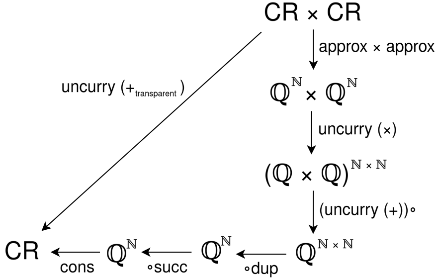
Figure 6: A possible transparent implementation of the sum of two CompReals (abbreviated as CR)
