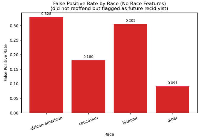
Fig. 7. FPR among race groups (race-blind model).
