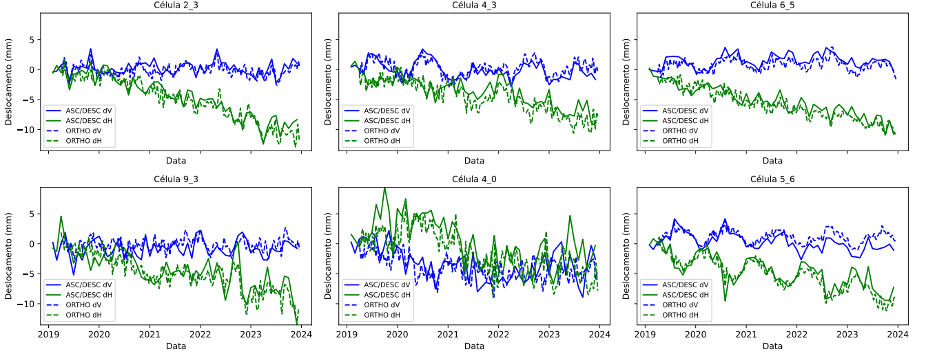
Figure 4: Time-series plots of dV and dH from ASC/DESC IDW compared to ORTHO.
