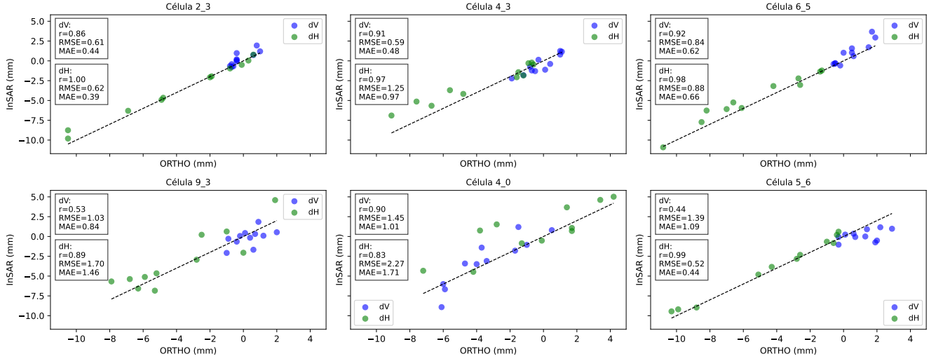
Figure 5: Local-scale correlation analysis for a representative sample of grid cells. Each panel displays the scatter plot between InSAR-derived and ORTHO displacements ( dV and dH ), including cell-specific error metrics (RMSE, MAE, and Pearson's r ).
