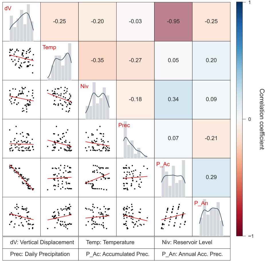
Figure 12: Multivariate correlation matrix for Cluster 2 (Right Abutment/Slopes).
