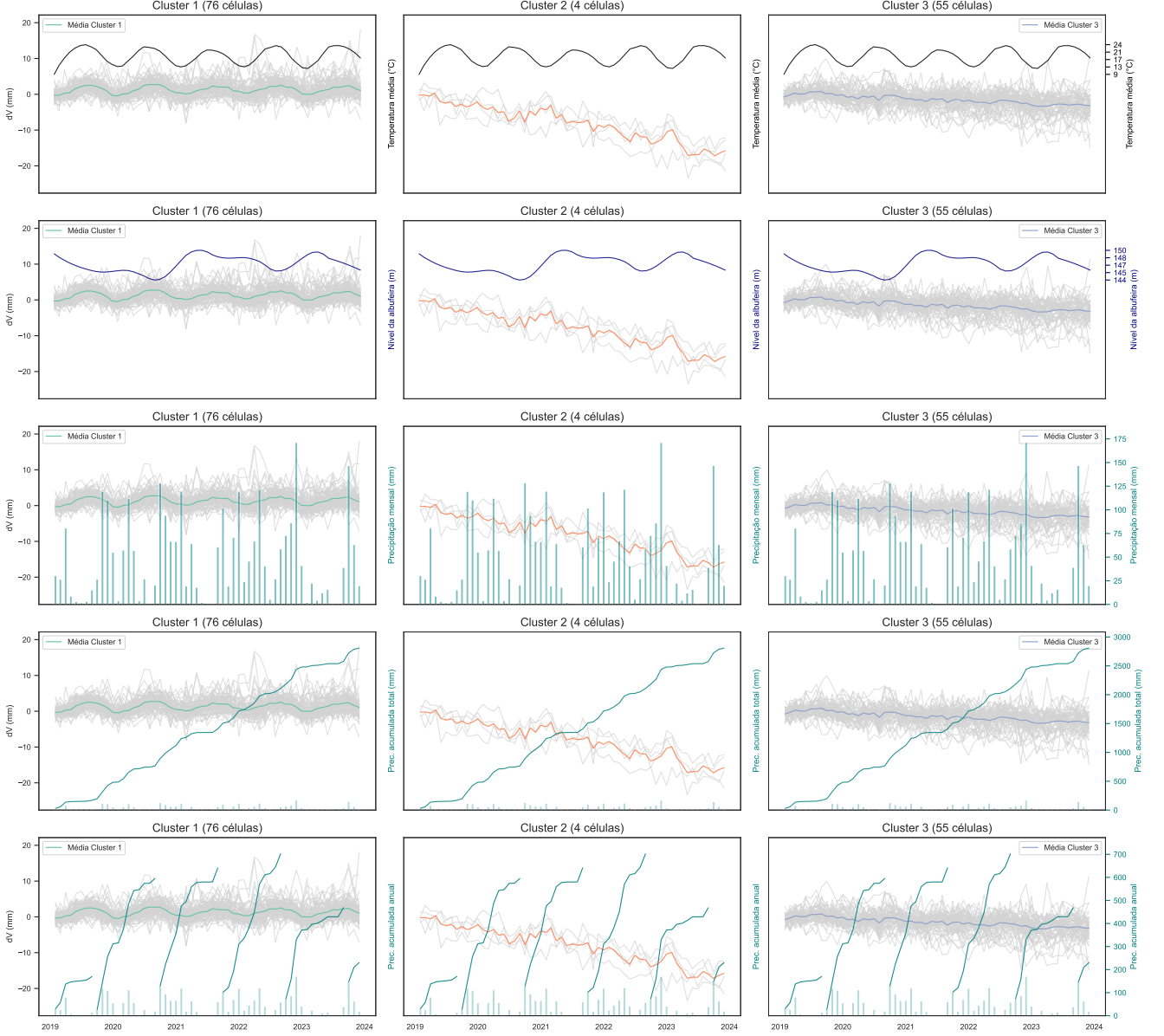
Figure 9: Multivariate analysis of vertical displacement ( dV ) time series per cluster. For each cluster, external environmental variables: Temperature, Reservoir Level, and Precipitation, are integrated.
