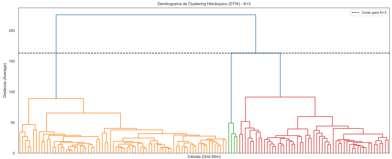
Figure 7: Dendrogram of the hierarchical clustering using DTW distance. The vertical axis represents the merging distance (dissimilarity). The dashed horizontal line indicates the automatic cut-off point determined by the Elbow method, resulting in the identification of K distinct clusters based on their deformation signatures
