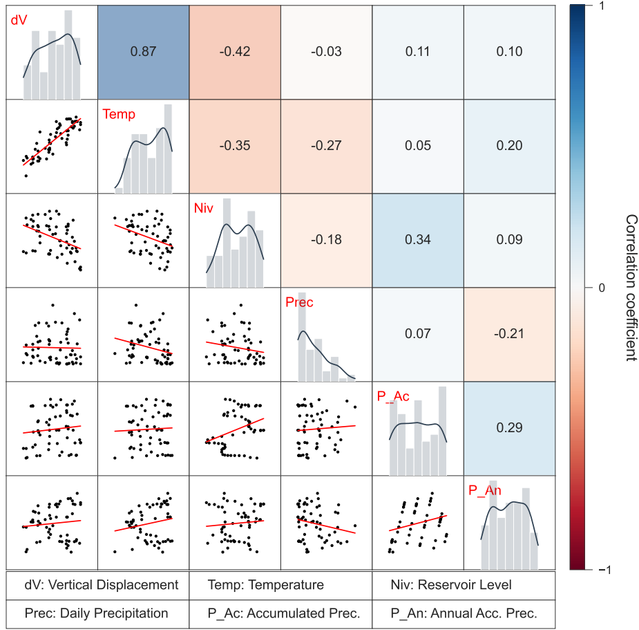
Figure 11: Multivariate correlation matrix for Cluster 1 (Main Dam Body).
