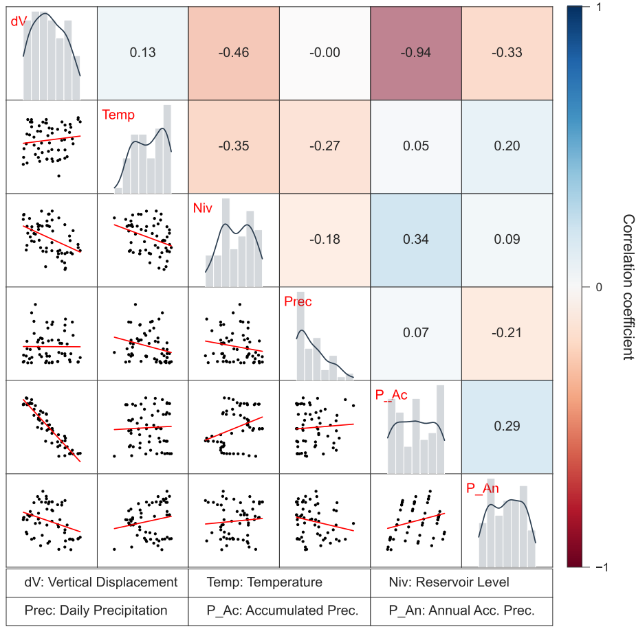
Figure 13: Multivariate correlation matrix (Pair Plot) for Cluster 3 (Left Abutment/Foundation).
