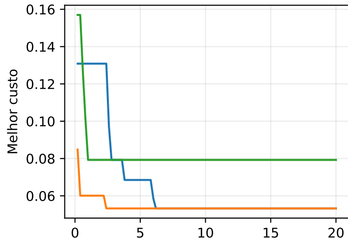
N=20, K=3
