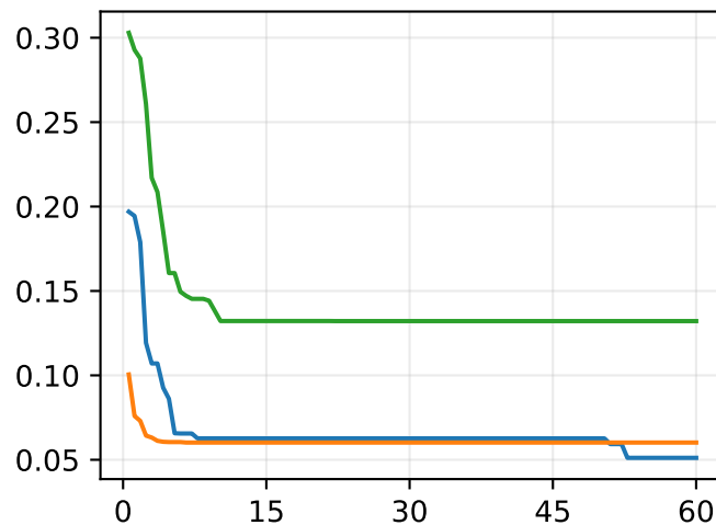
N=60, K=3
