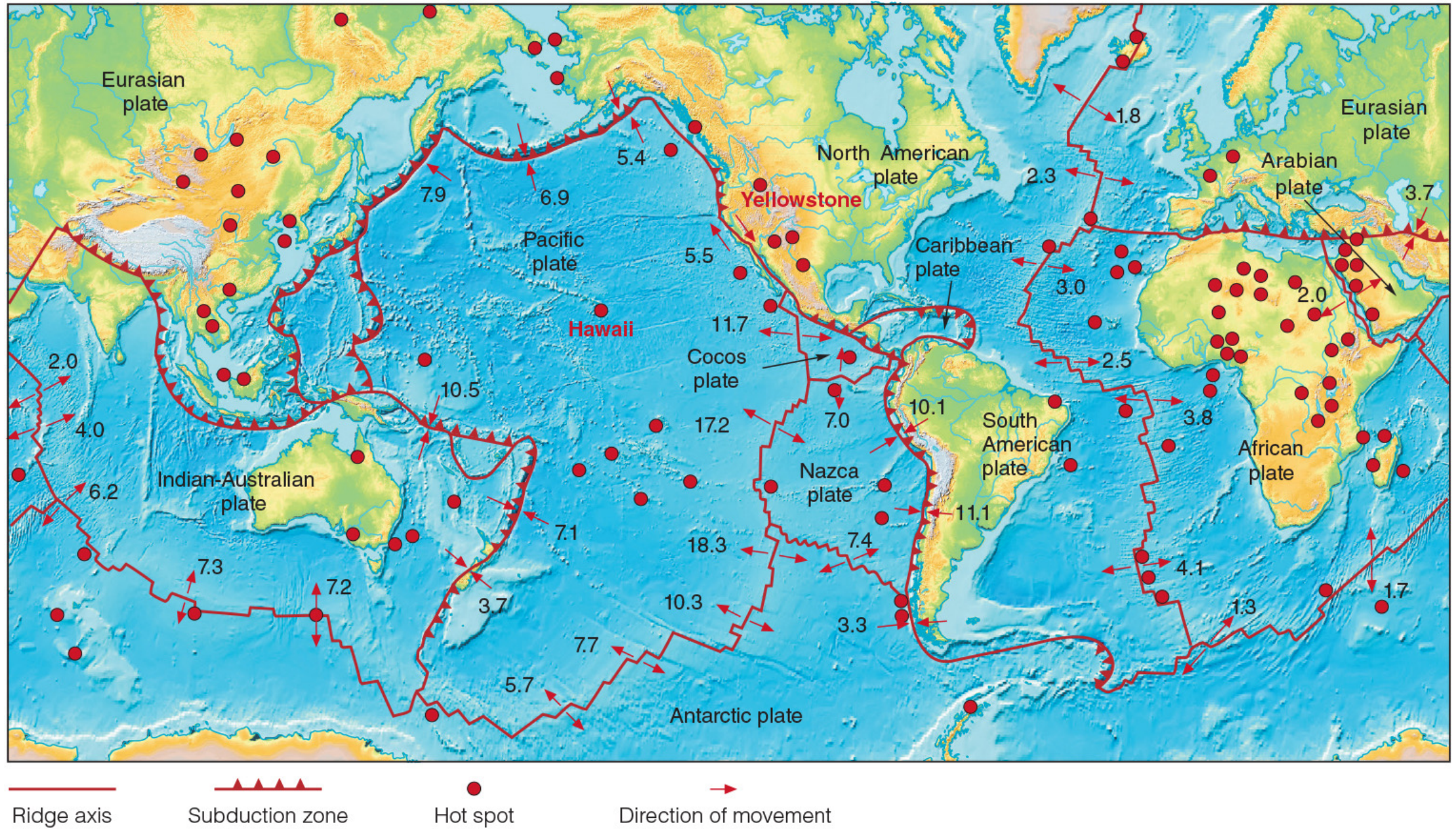
Figure 3.16 The major lithospheric plates, showing their directions of relative movement and speed as well as the location of the principal hot spots. Note the correspondence of plate boundaries and earthquake locations—compare this figure to Figure 3.15. Most of the million or so earthquakes and volcanic events each year occur along plate boundaries.
