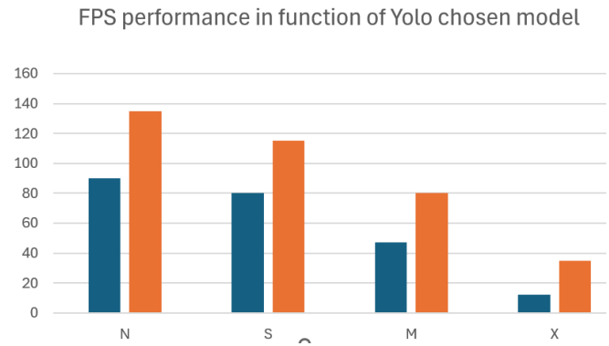
Fig. 14. FPS performance comparison: .pytorch (blue) vs .engine (orange)
