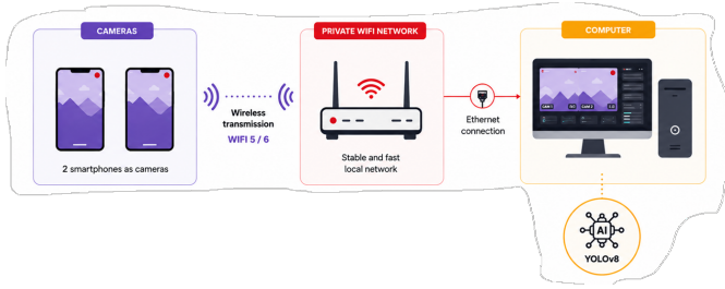
Fig. 9. Network topology: two smartphones transmit wirelessly via HTTP to a private Wi-Fi router, which forwards data via gigabit Ethernet to the processing computer.
