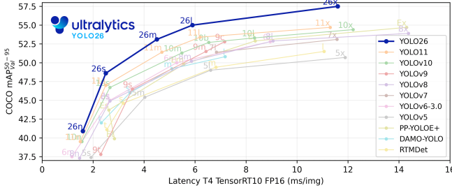
Fig. 5. Comparison of YOLO models [19]
