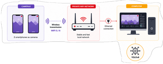
Fig. 9. Network topology: two smartphones transmit wirelessly via HTTP to a private Wi-Fi router, which forwards data via gigabit Ethernet to the processing computer.
