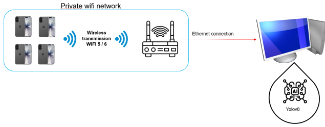
Fig. 6. Network topology: four smartphones transmit wirelessly via HTTP (80 m range) to a private Wi-Fi router, which forwards data via gigabit Ethernet to the YOLOv8 processing computer.
