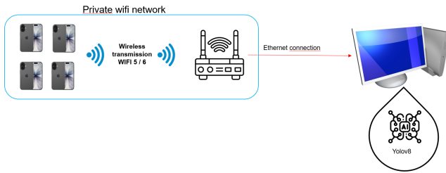
Fig. 7. Network topology: four smartphones transmit wirelessly via HTTP (80m range) to a private Wi-Fi router, which forwards data via gigabit Ethernet to the YOLOv8 processing computer.
