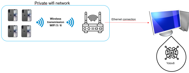
Fig. 4. Network topology: four smartphones transmit wirelessly via HTTP (80m range) to a private Wi-Fi router, which forwards data via gigabit Ethernet to the YOLOv8 processing computer.
