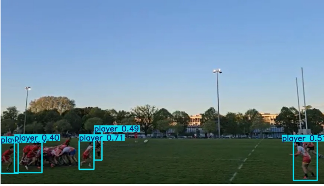
Fig. 11. Test image 2, used trained yolov8n model.
