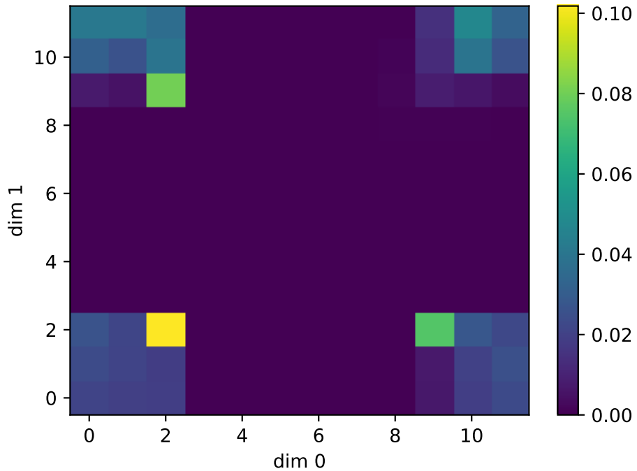
Learned (GFN)
