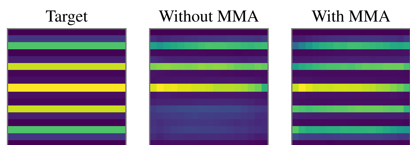
Figure 3: Lazy Random Walk : MMA recovers the striped target the un-augmented sampler washes out.
