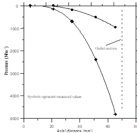
Figure 1. Pressure variation along the nozzle: experimental data
