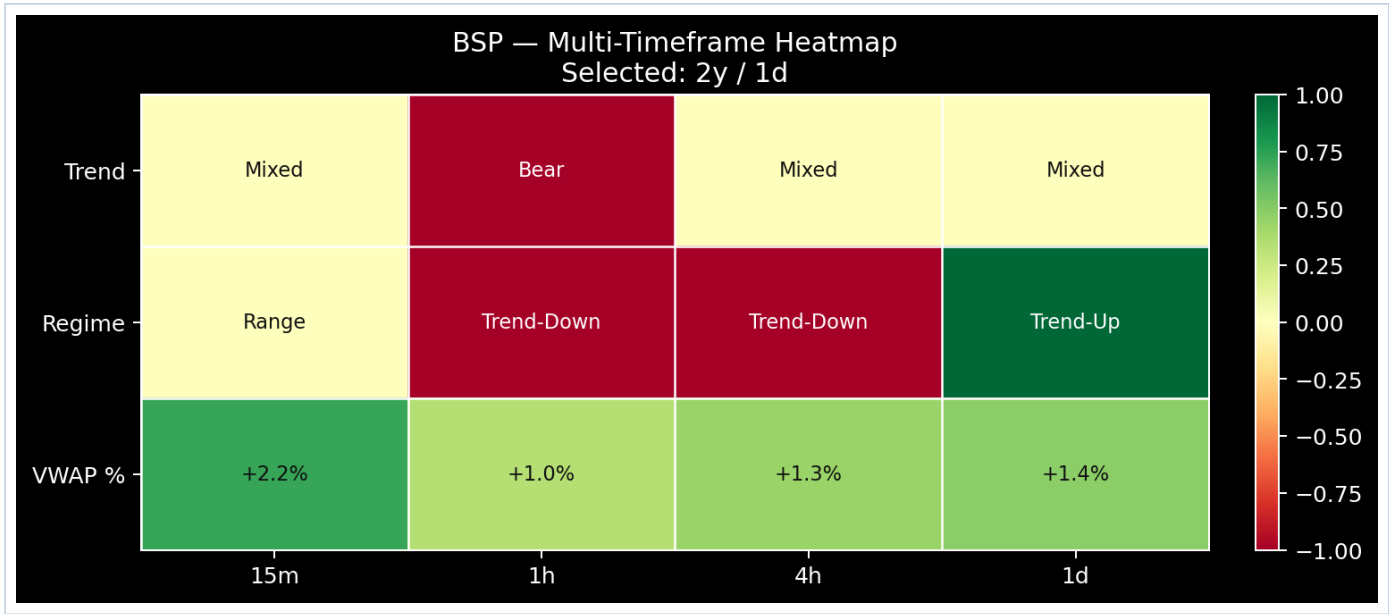
Figure 10. Multi-Timeframe Heatmap
