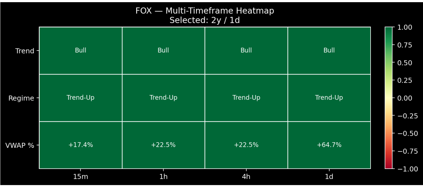
Figure 13. Multi-Timeframe Heatmap
