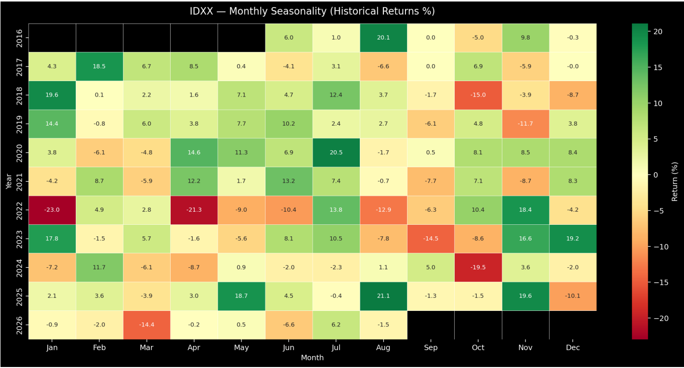
Figure 26. Monthly Seasonality Heatmap (10Y) As-of: 2026-08-14
