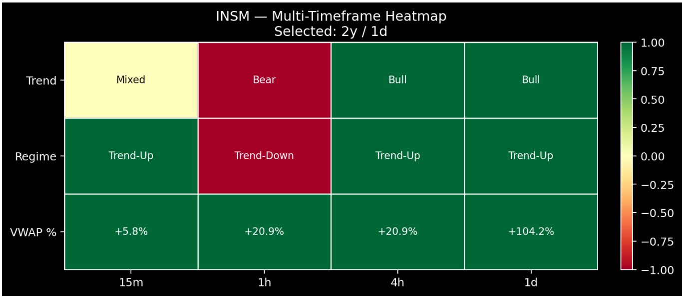
Figure 14. Multi-Timeframe Heatmap
