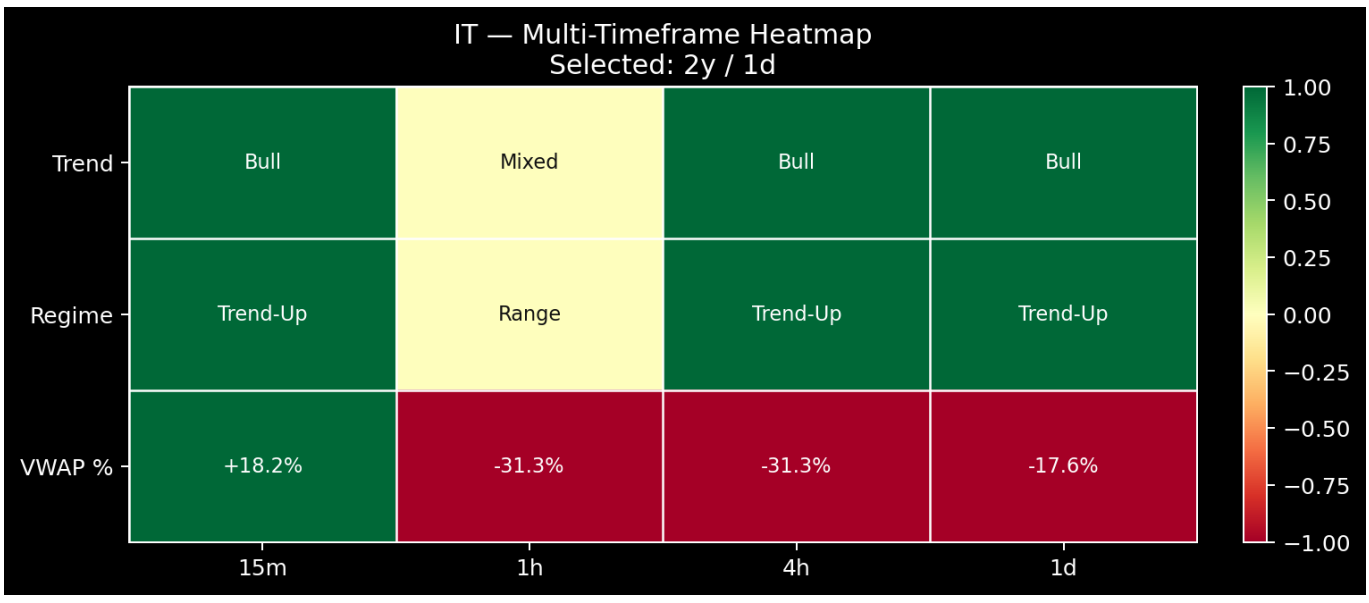
Figure 14. Multi-Timeframe Heatmap
