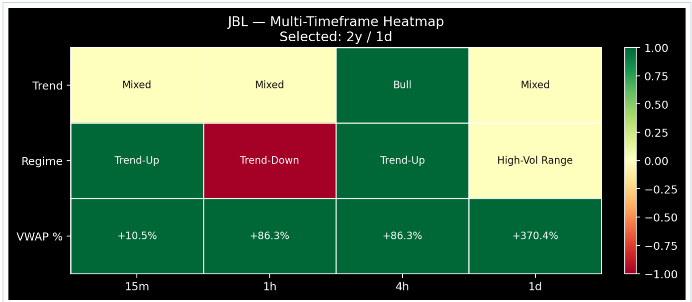
Figure 12. Multi-Timeframe Heatmap
