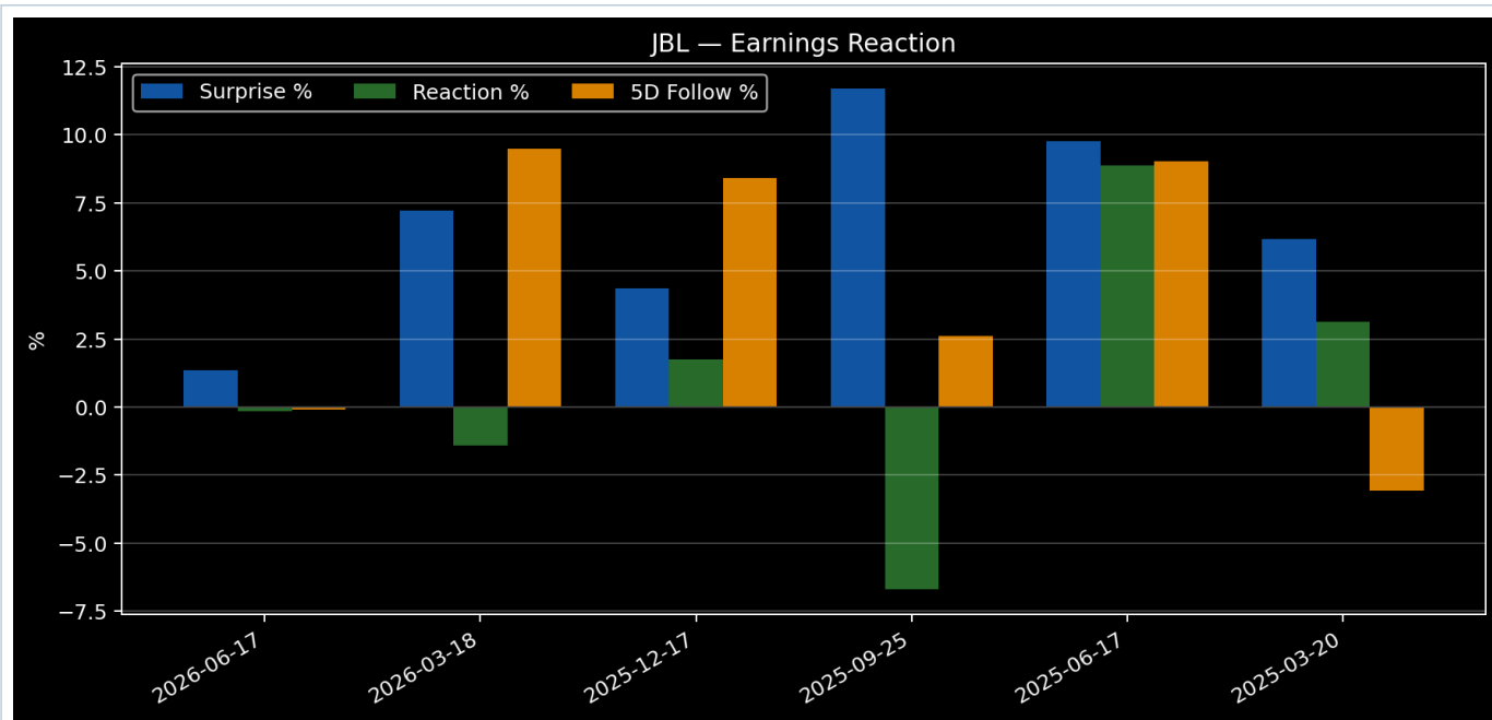
Figure 21. Earnings Reaction
