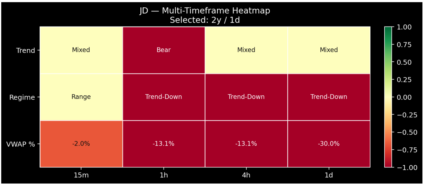
Figure 10. Multi-Timeframe Heatmap
