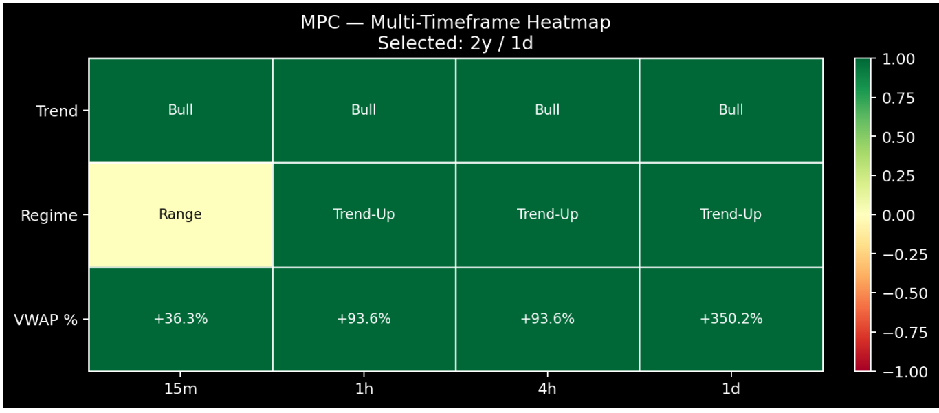
Figure 14. Multi-Timeframe Heatmap
