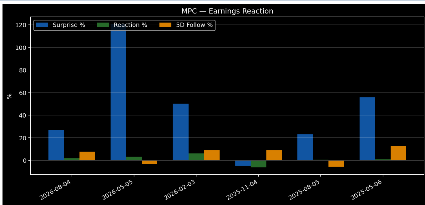
Figure 22. Earnings Reaction
