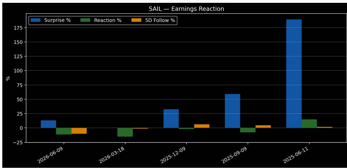
Figure 23. Earnings Reaction
