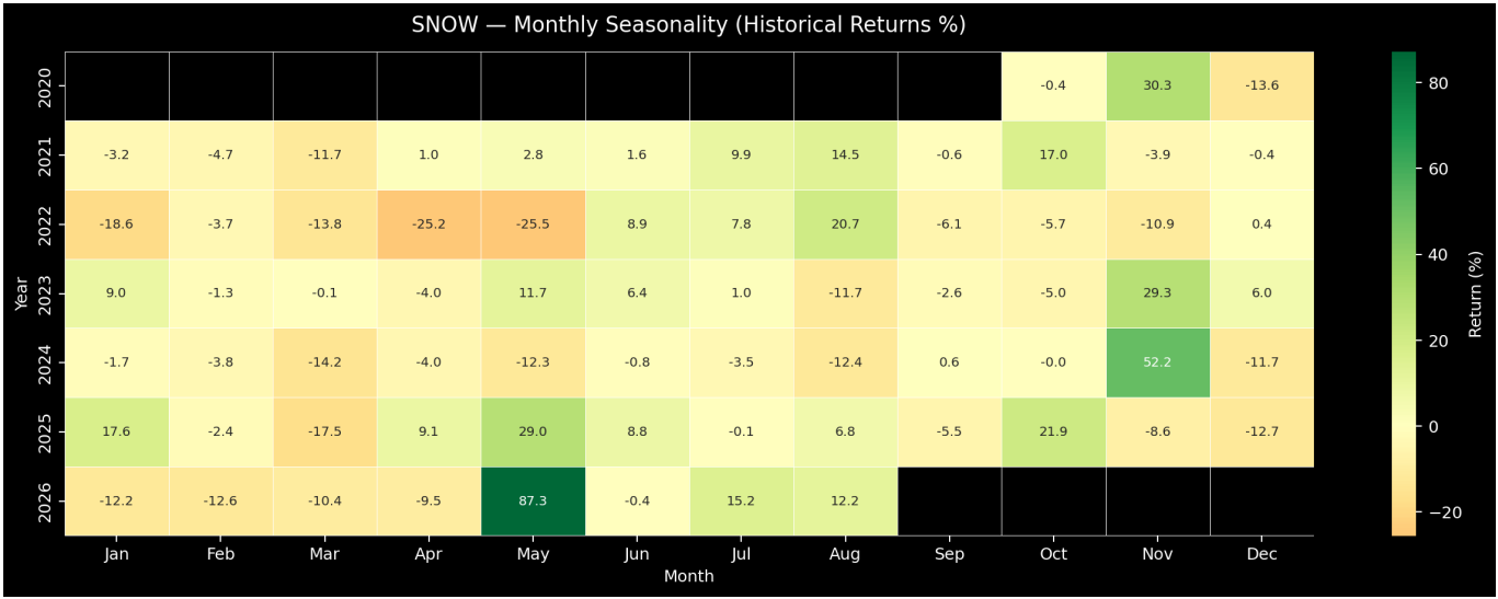
Figure 28. Monthly Seasonality Heatmap (10Y) As-of: 2026-08-14
