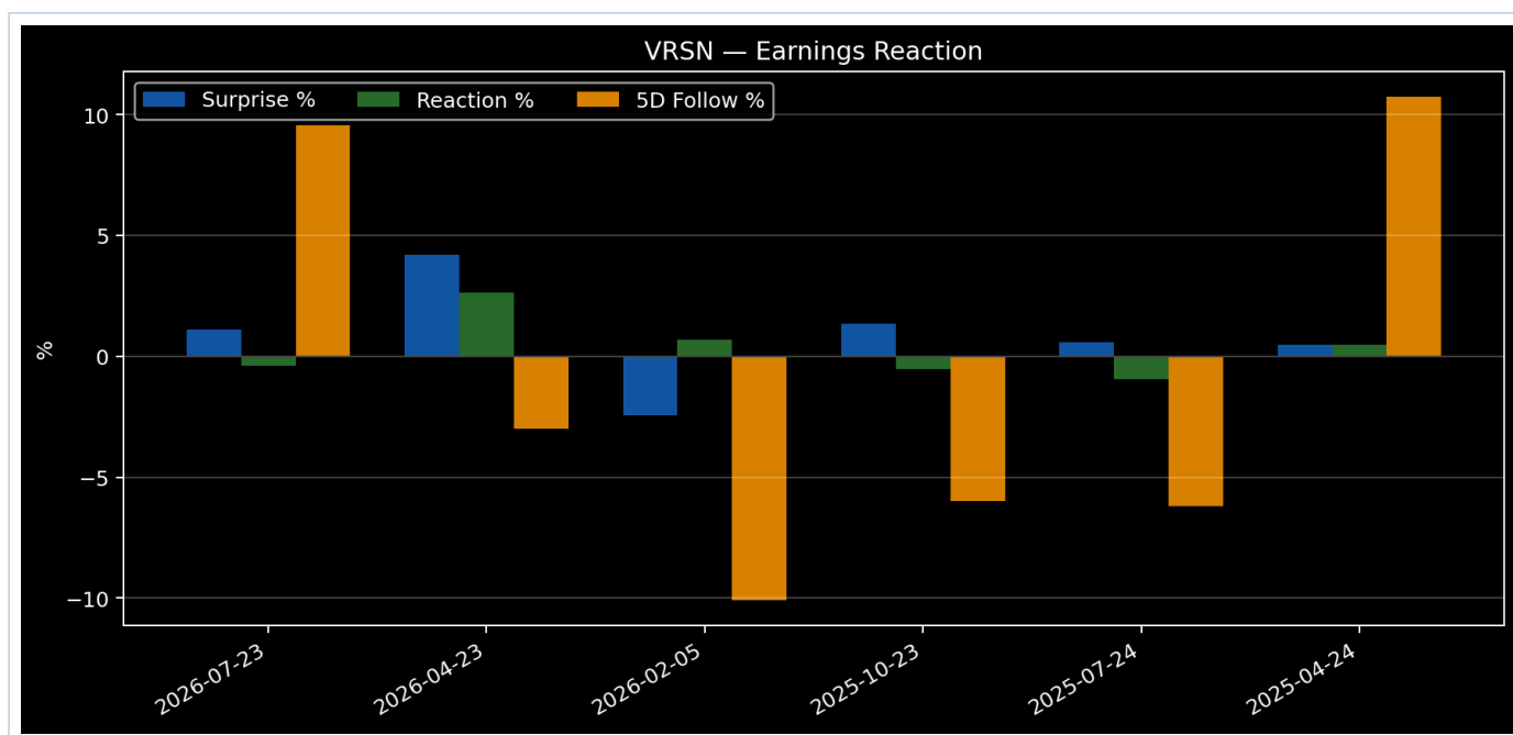
Figure 23. Earnings Reaction
