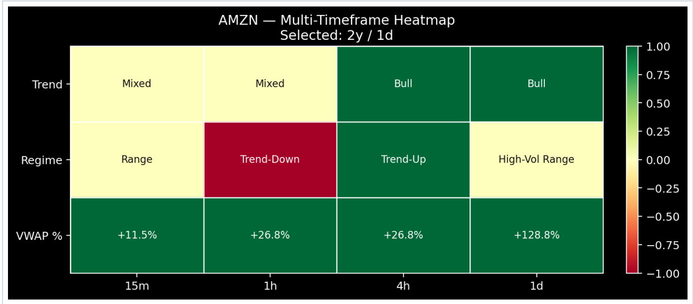
Figure 13. Multi-Timeframe Heatmap
