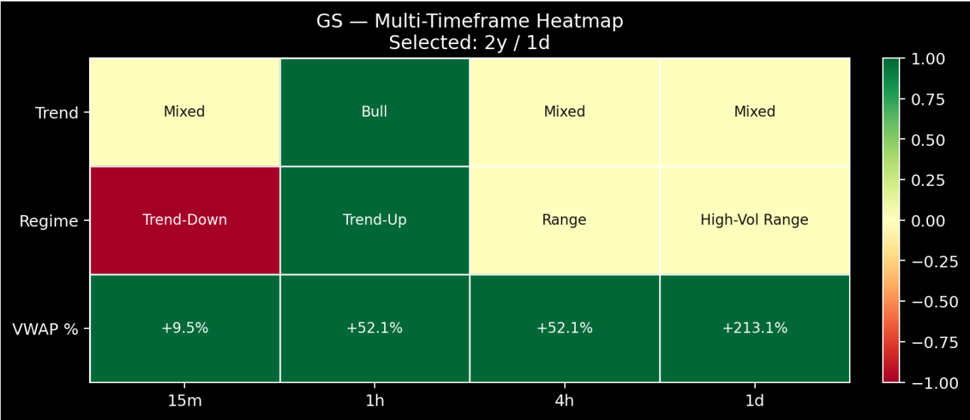
Figure 13. Multi-Timeframe Heatmap
