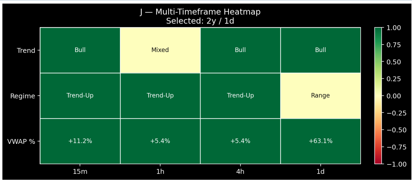
Figure 12. Multi-Timeframe Heatmap
