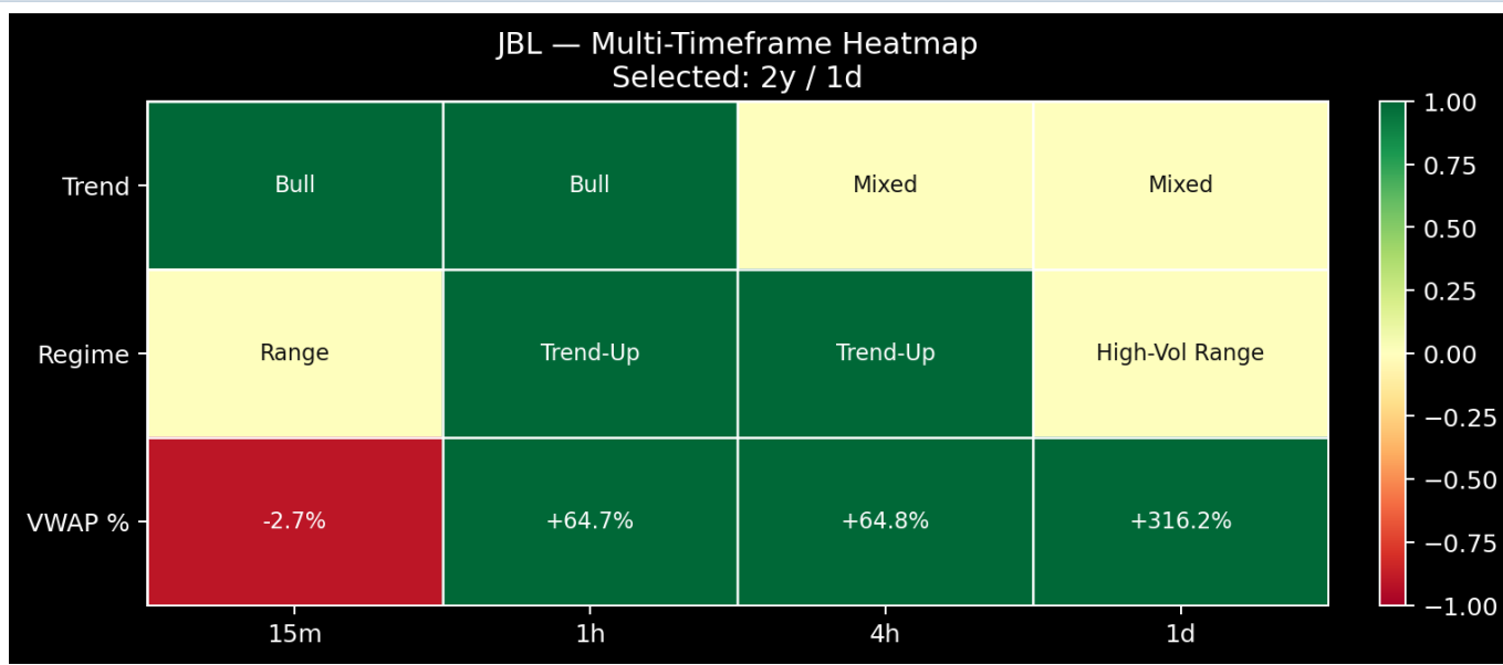
Figure 12. Multi-Timeframe Heatmap
