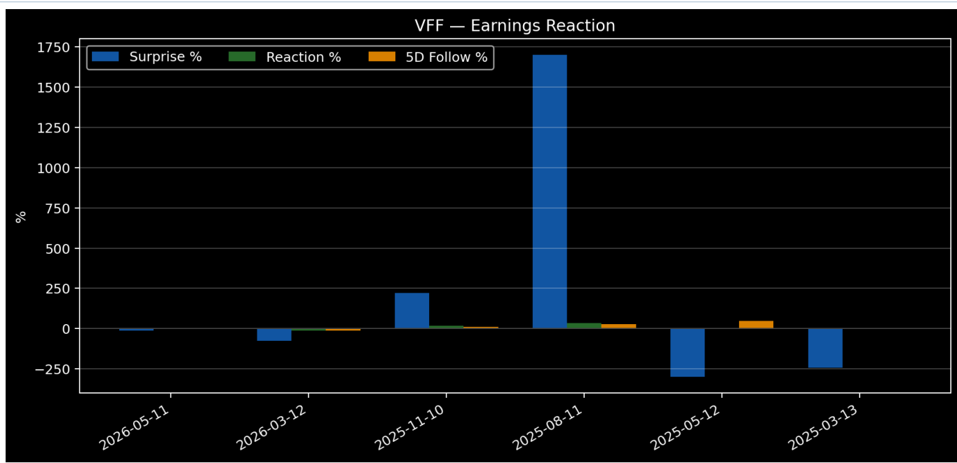
Figure 15. Earnings Reaction
