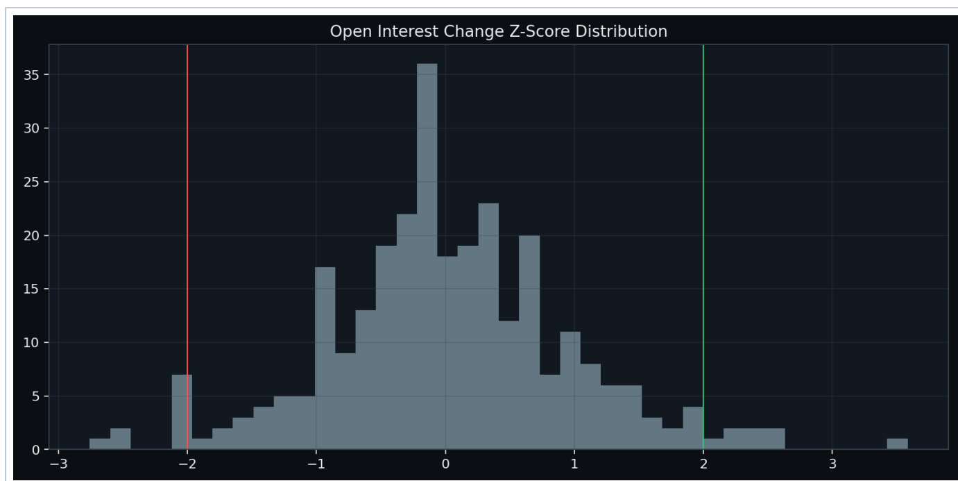
Figure 2. Distribution of 20-day OI change z-scores
