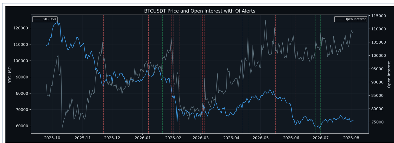
Figure 1. BTCUSDT BTC-USD price and open interest with signals
