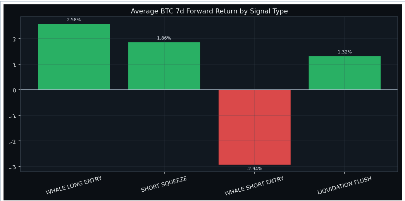
Figure 3. Average BTC 7d forward return by signal type
