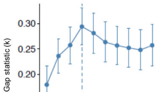
Gap statistic
